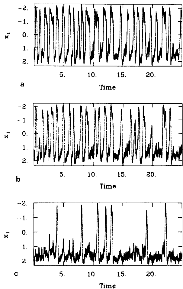
Fig. 6 a–c. Trace of the x_1 variable of a Monte Carlo trajectory for the stochastic Bonhoeffer-van der Pol model with \beta = 10 representing the electrical membrane potential of a neuron; a z = -0.4 (limit cycle situation), b z = 0 (no limit cycle), c z = 1 (no limit cycle)
