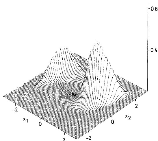
Fig. 3. Stationary distribution of the stochastic Bonhoeffer-van der Pol model with z = -0.4 for the noise level \beta = 10 ; the distributions resulted from single Monte Carlo trajectories sampling about 29 000 000 points (Treutlein and Schulten 1985)
