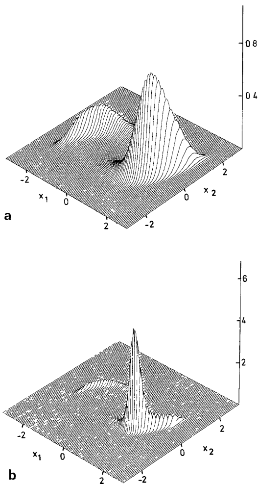
Fig. 4 a and b. Stationary distribution of the stochastic Bonhoeffer-van der Pol model for z=0 , i.e. the case that no deterministic limit cycle exists; the distributions results from a Monte Carlo trajectory sampling about 29 000 000 jump points; a \beta = 10 , b \beta = 100 (Treutlein and Schulten 1985)
